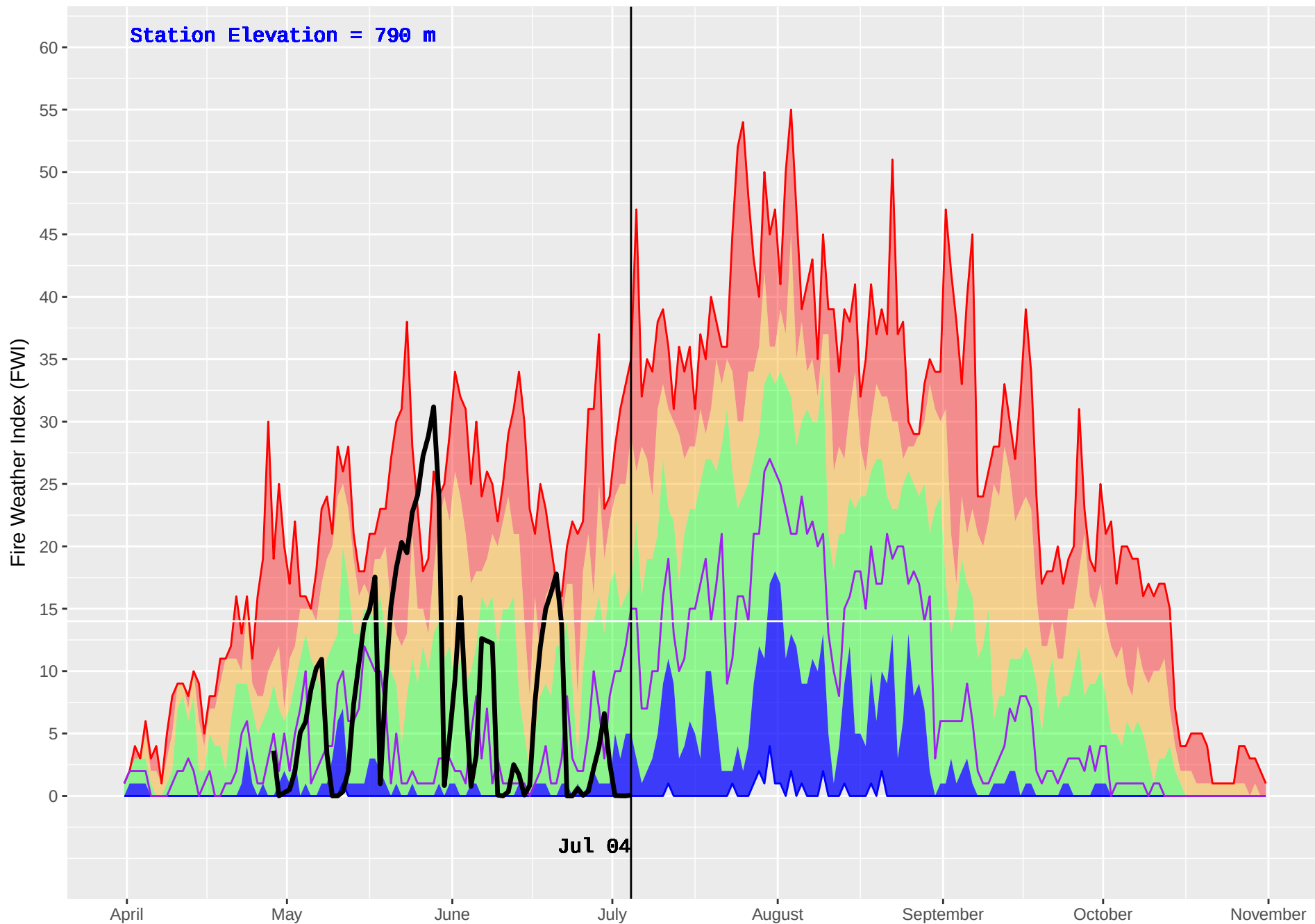
FALLS CREEK (383) : Historical (2002–2016) and Current (2018) Noon Fire Weather Index (FWI)
