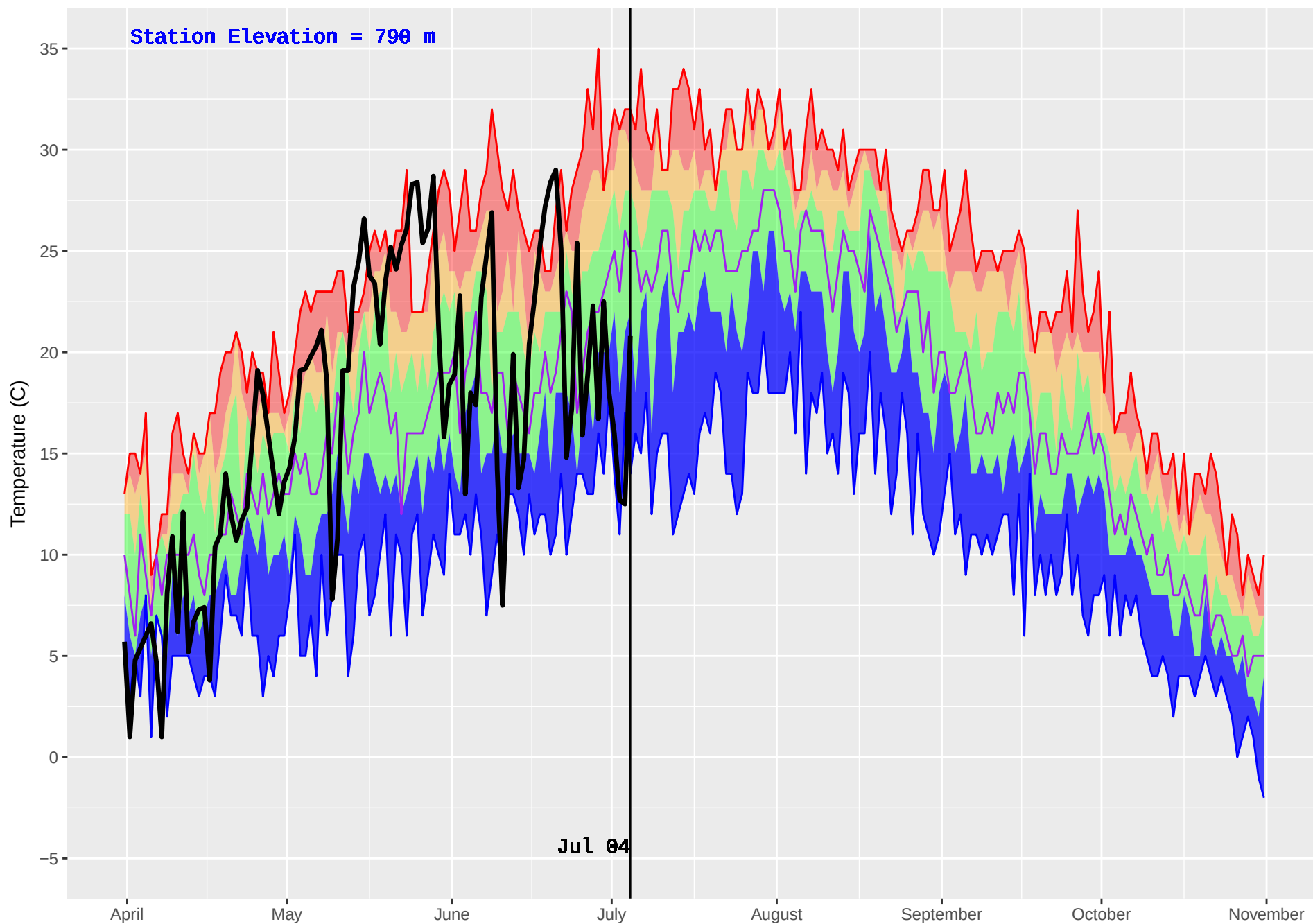
FALLS CREEK (383) : Historical (2002–2016) and Current (2018) Noon Temperature
